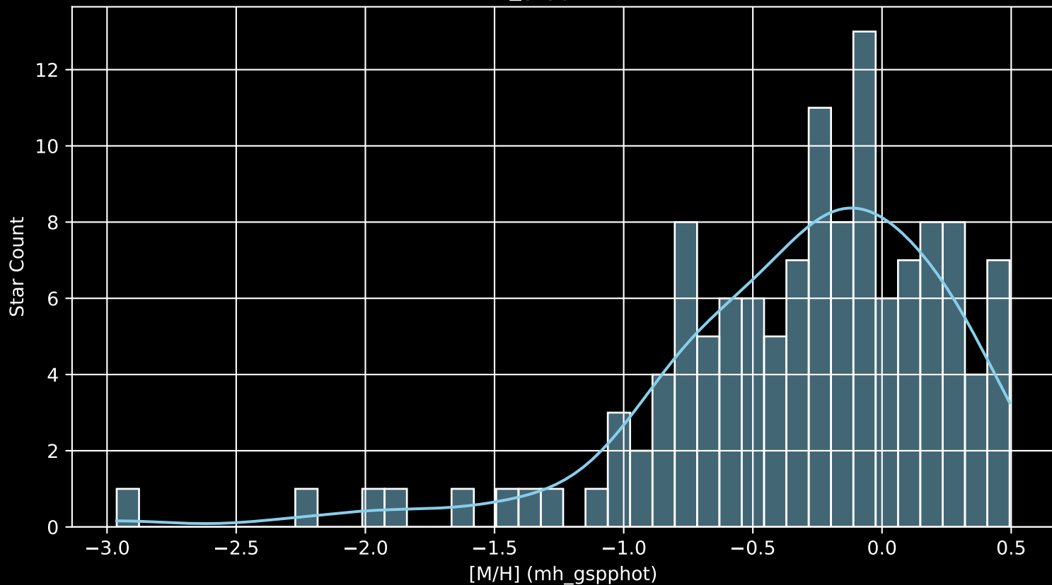
APOGEE DR17 Field: [020+02 [M/H] (mh_gspphot) (n= 127)
