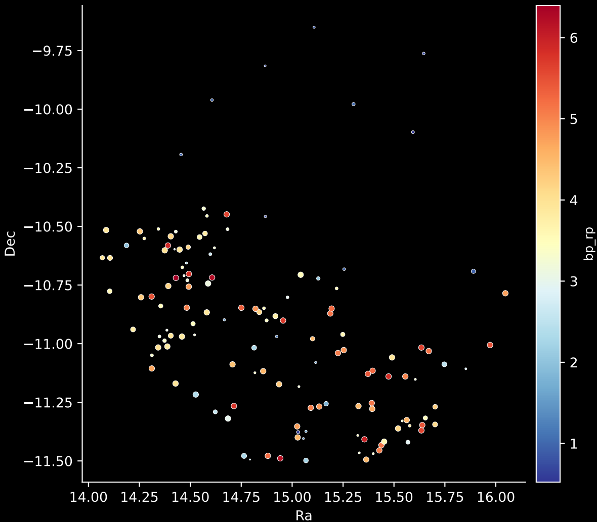
APOGEE DR17 Field: [020+02] Stars: 137
