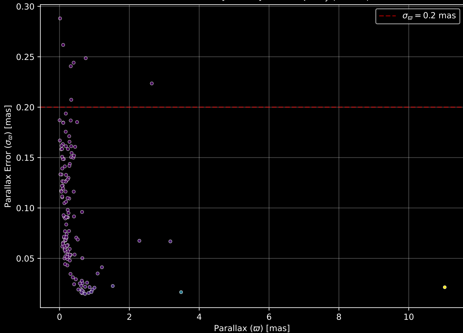
APOGEE DR17 Field: [020+02] Parallax Quality (n= 137)
