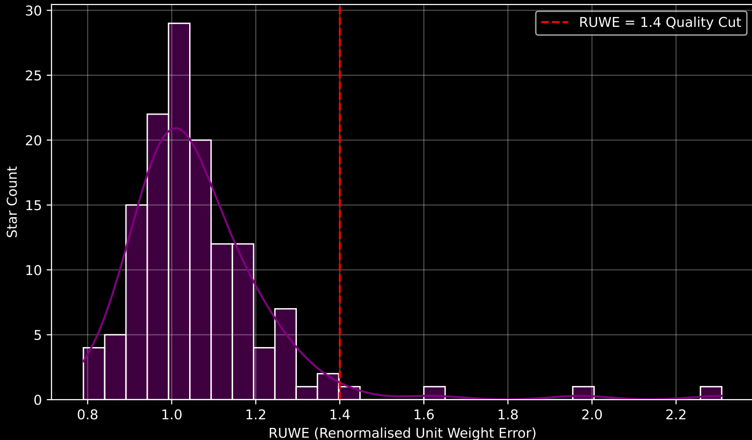
GAPOGEE DR17 Field [020+02] RUWE Distribution (n= 137)
