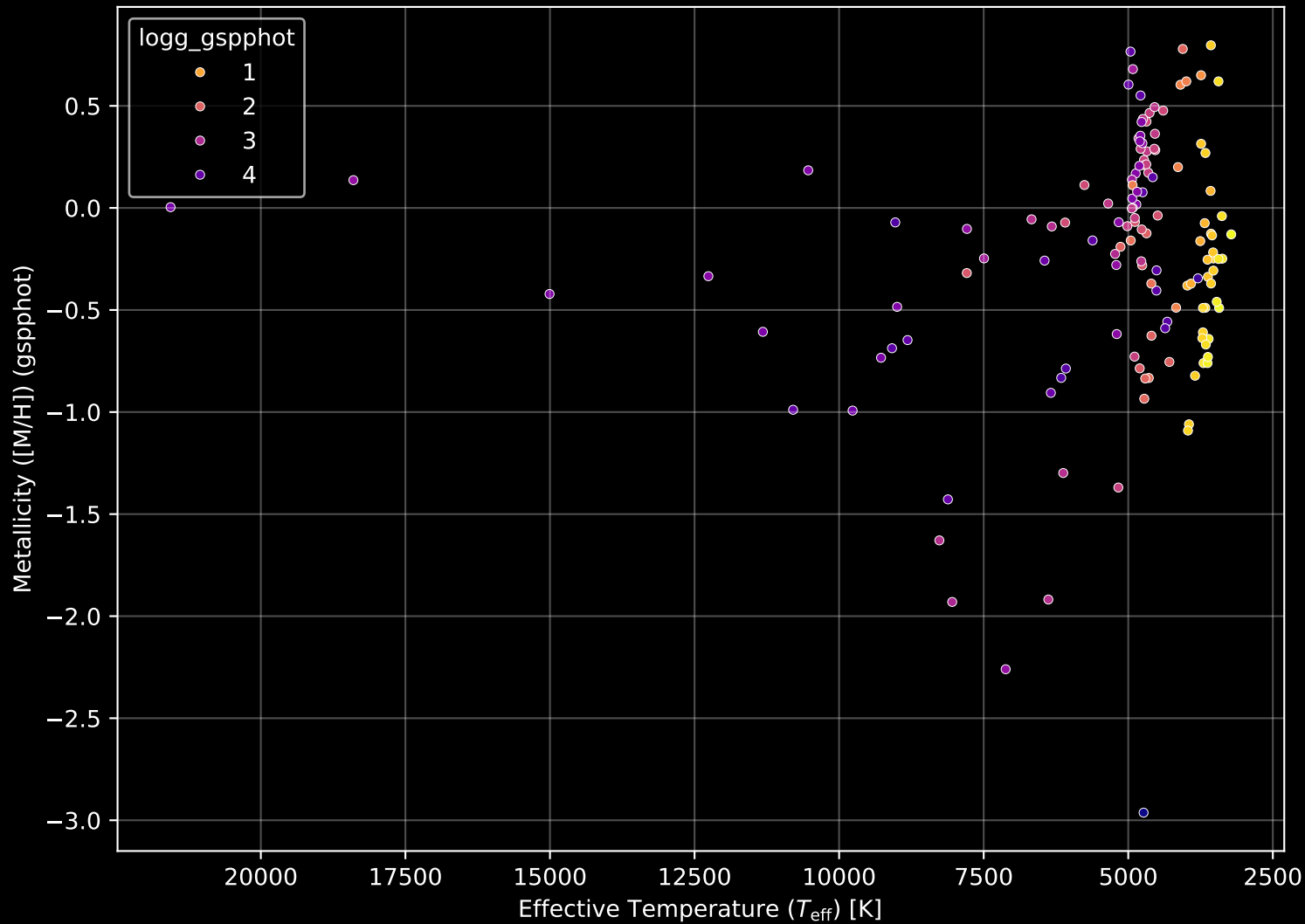
APOGEE DR17 Field: [020+02] Stellar Population Parameters (n= 137)
