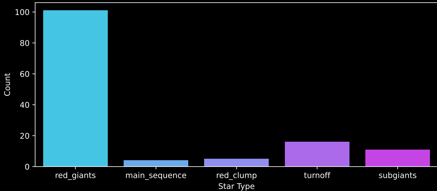
APOGEE DR17 Field: [020+02] Count plot of Star Type
