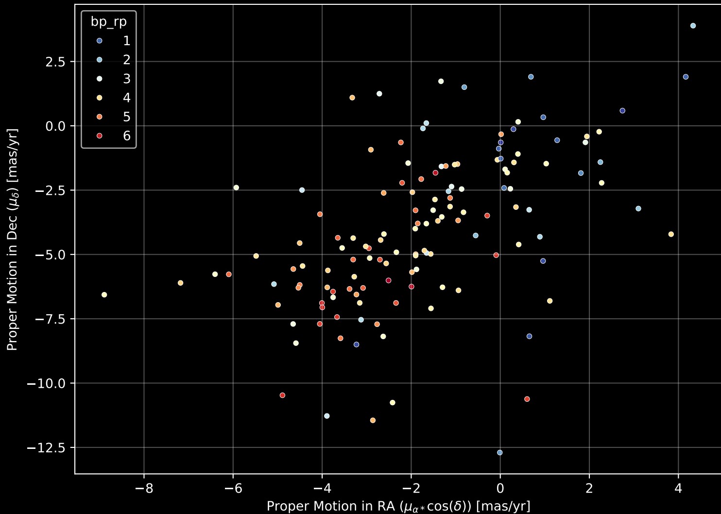
APOGEE DR17 Field: [020+02] Proper Motion Diagram (n= 137)
